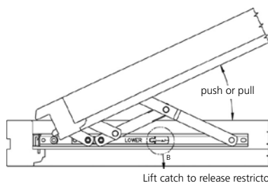
Lift catch to release restrictor
