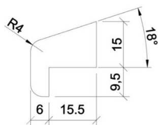
Figure 5 – Meranti Bead
