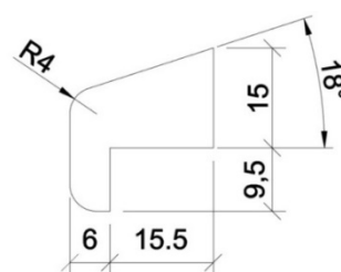
Figure 6 – MDF Bead
