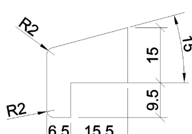
Figure 4 – MDF Bead – Option 3
