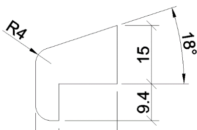
Figure 3 – MDF Bead – Option 2
