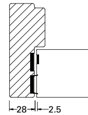
Detail top frame
