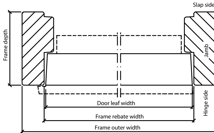
Door outwards opening
