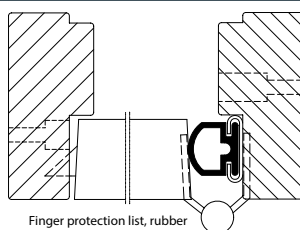
Finger protection list, rubber
