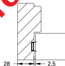
Detail top frame
