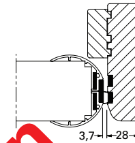
Single door, stop side
