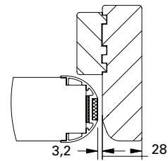
Single door, stop side
