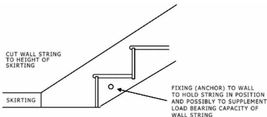
Figure 3 – Bottom of wall string to floor
