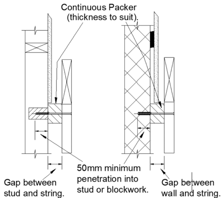
Figure 1a. Section through wall string at stud wall and blockwork
