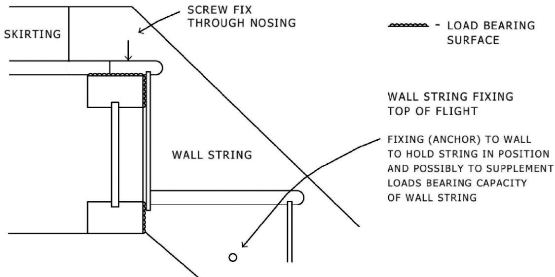
Figure 2 – Top of wall string
