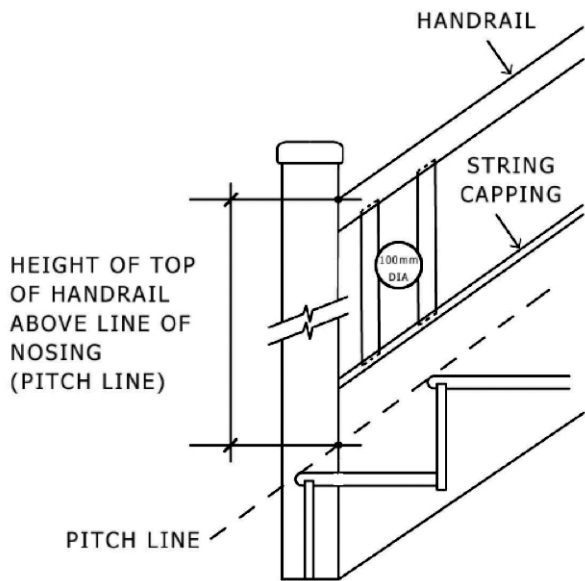
Figure 10 – Newel, balusters, handrail etc.
