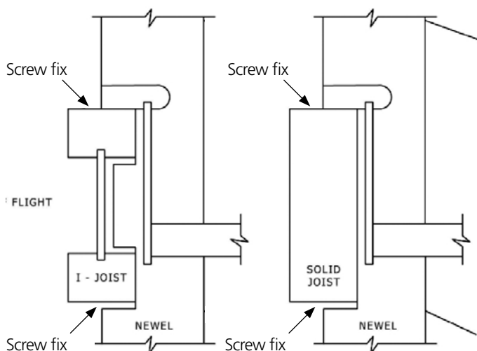
Figure 5 – Top of outer string
