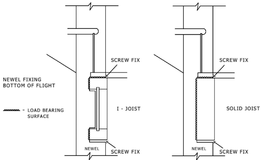
Figure 7 – Bottom treads - side view
